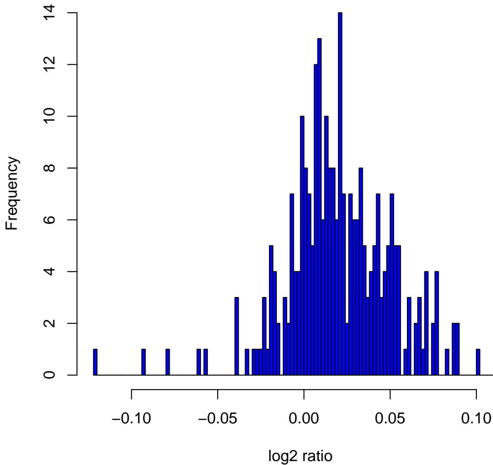
Histogram of log 2 ratios in 270 HapMap samples at clone Chr6tp-9G9
