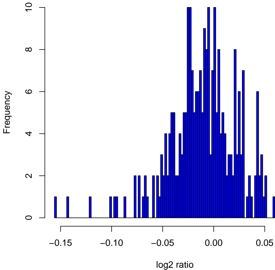
Histogram of log 2 ratios in 270 HapMap samples at clone Chr6tp-9H2
