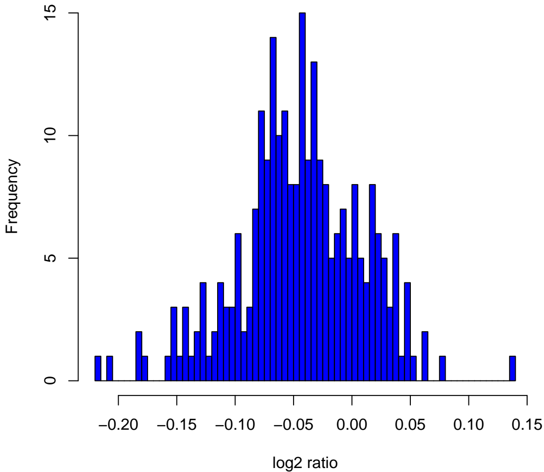
Histogram of log 2 ratios in 270 HapMap samples at clone Chr6tp-9H8
