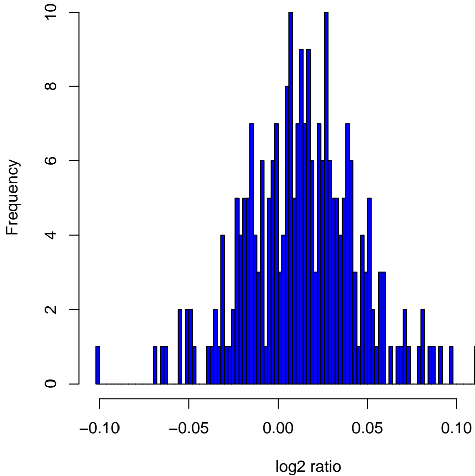
Histogram of log2ratios in 270 HapMap samples at clone Chr18tp-2H11
