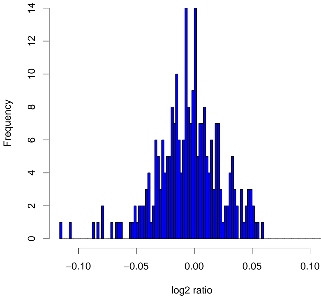
Histogram of log 2 ratios in 270 HapMap samples at clone Chr7tp-10B7
