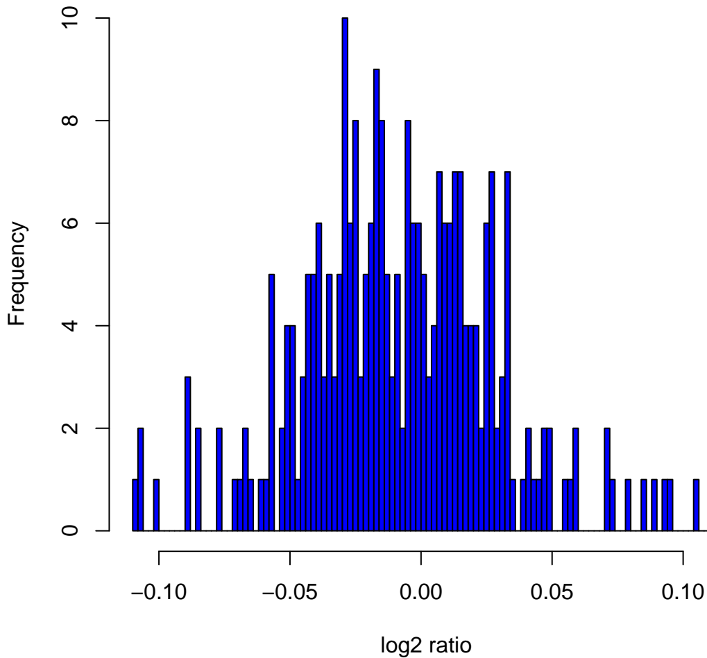
Histogram of log2ratios in 270 HapMap samples at clone Chr7tp-10G10
