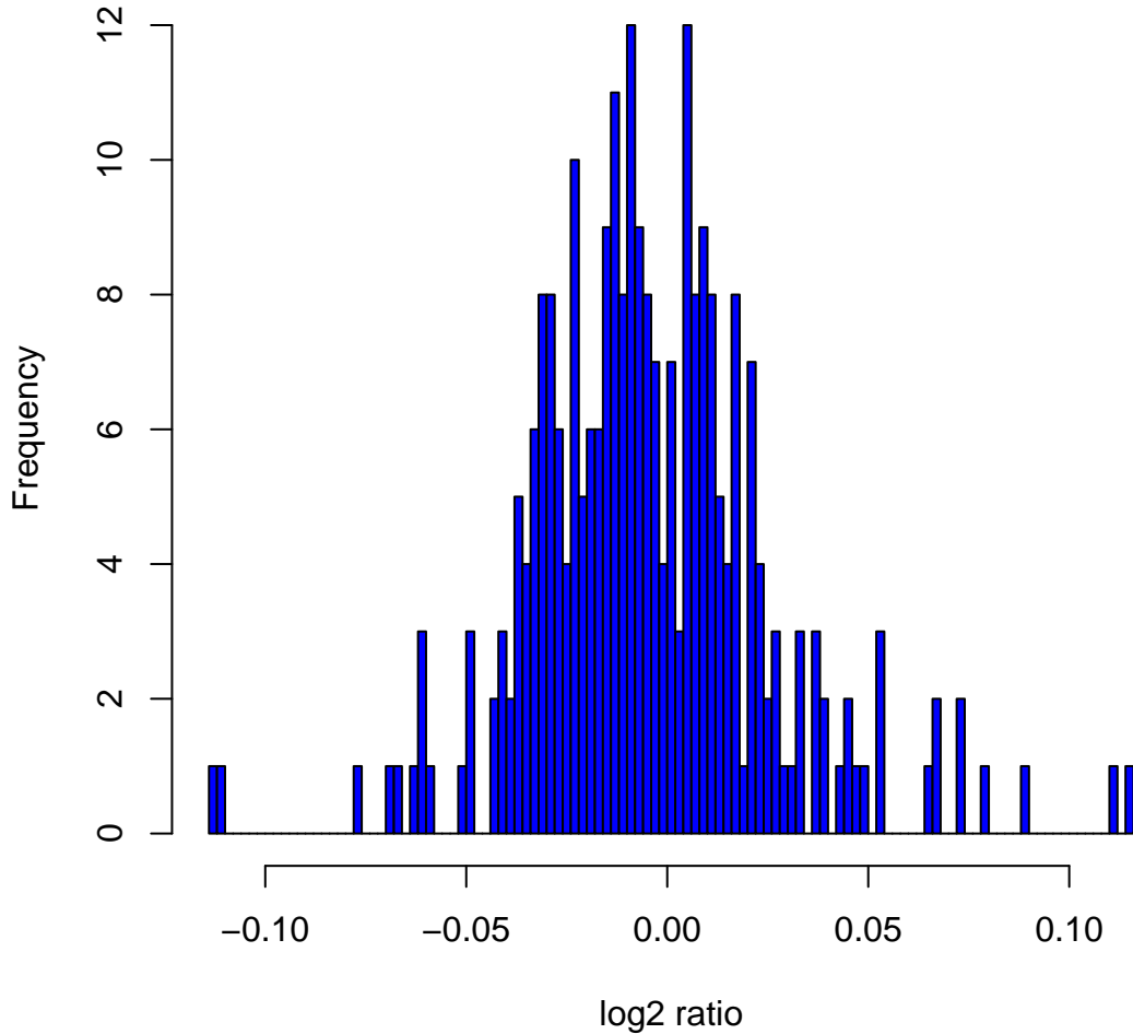
Histogram of log 2 ratios in 270 HapMap samples at clone Chr7tp-10G2
