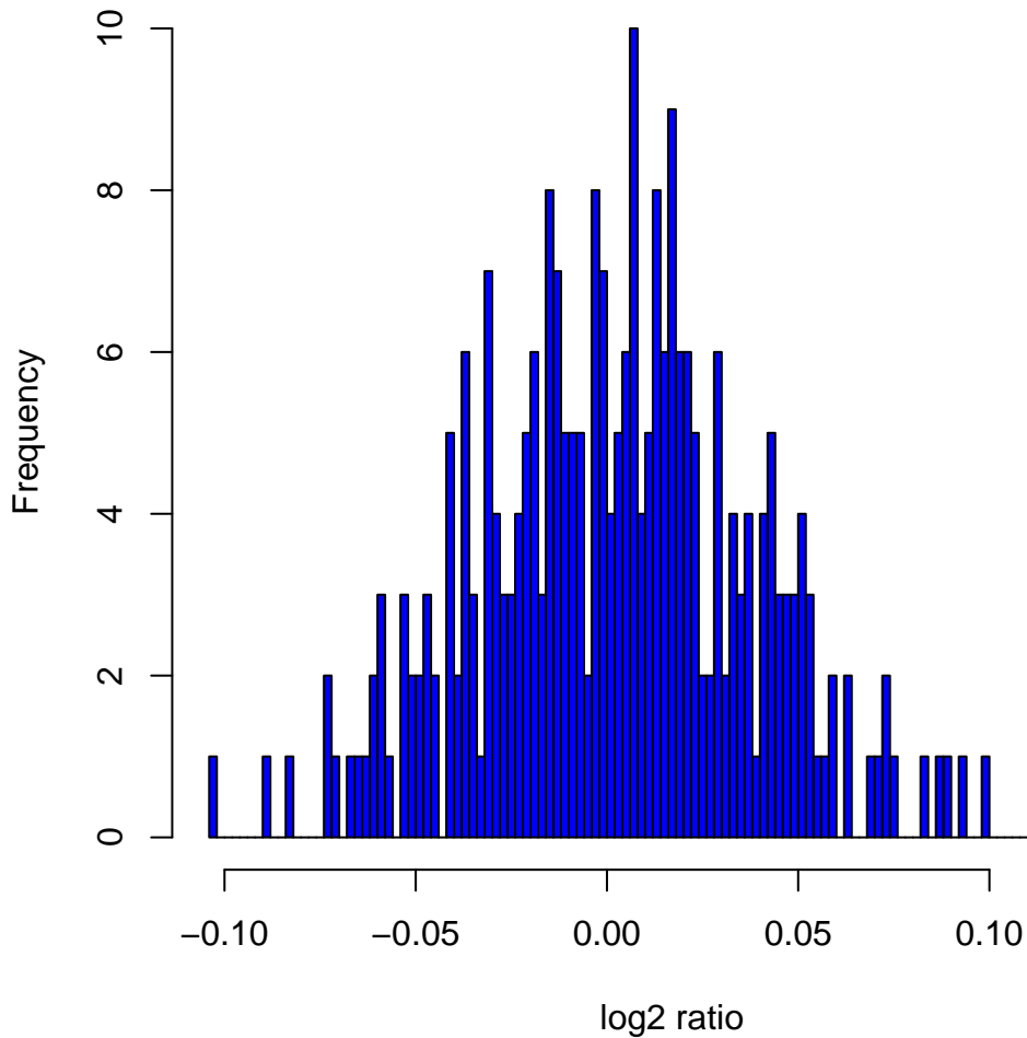
Histogram of log2ratios in 270 HapMap samples at clone Chr7tp-10H11
