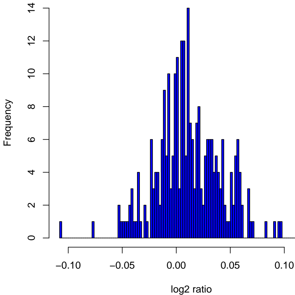
Histogram of log2ratios in 270 HapMap samples at clone Chr7tp-10H12
