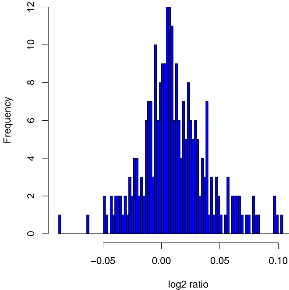
Histogram of log 2 ratios in 270 HapMap samples at clone Chr7tp-11B7
