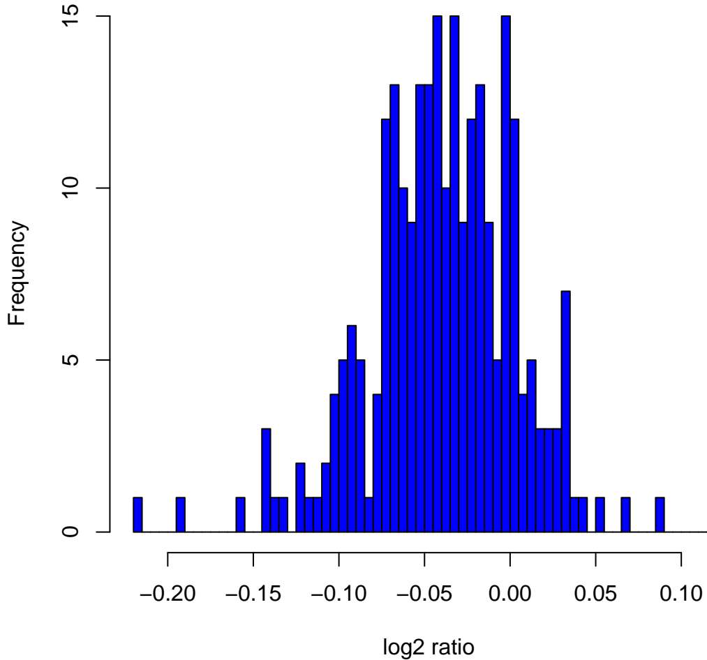
Histogram of log 2 ratios in 270 HapMap samples at clone Chr7tp-11D3
