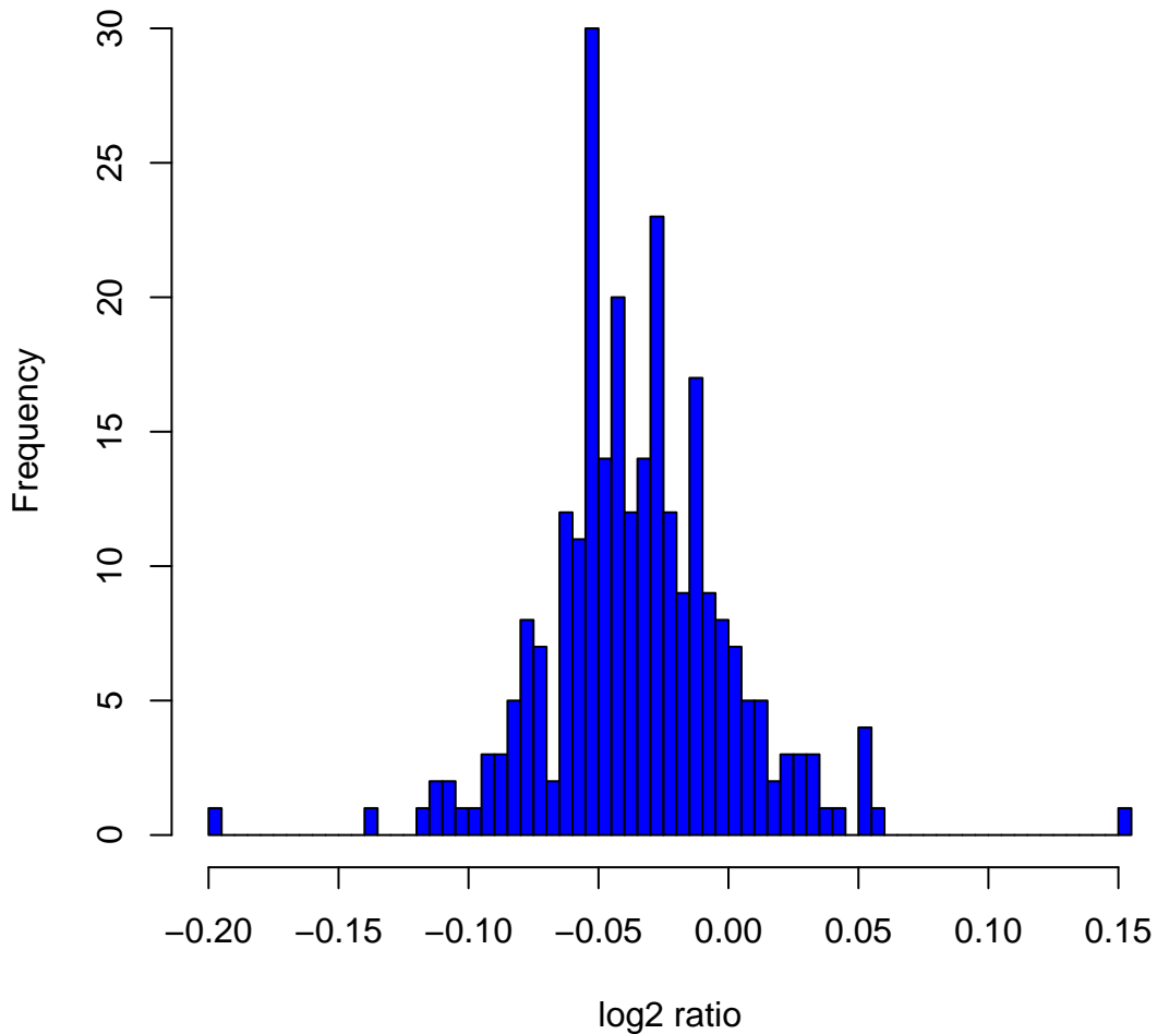
Histogram of \log_2 ratios in 270 HapMap samples at clone Chr7tp-11G9
