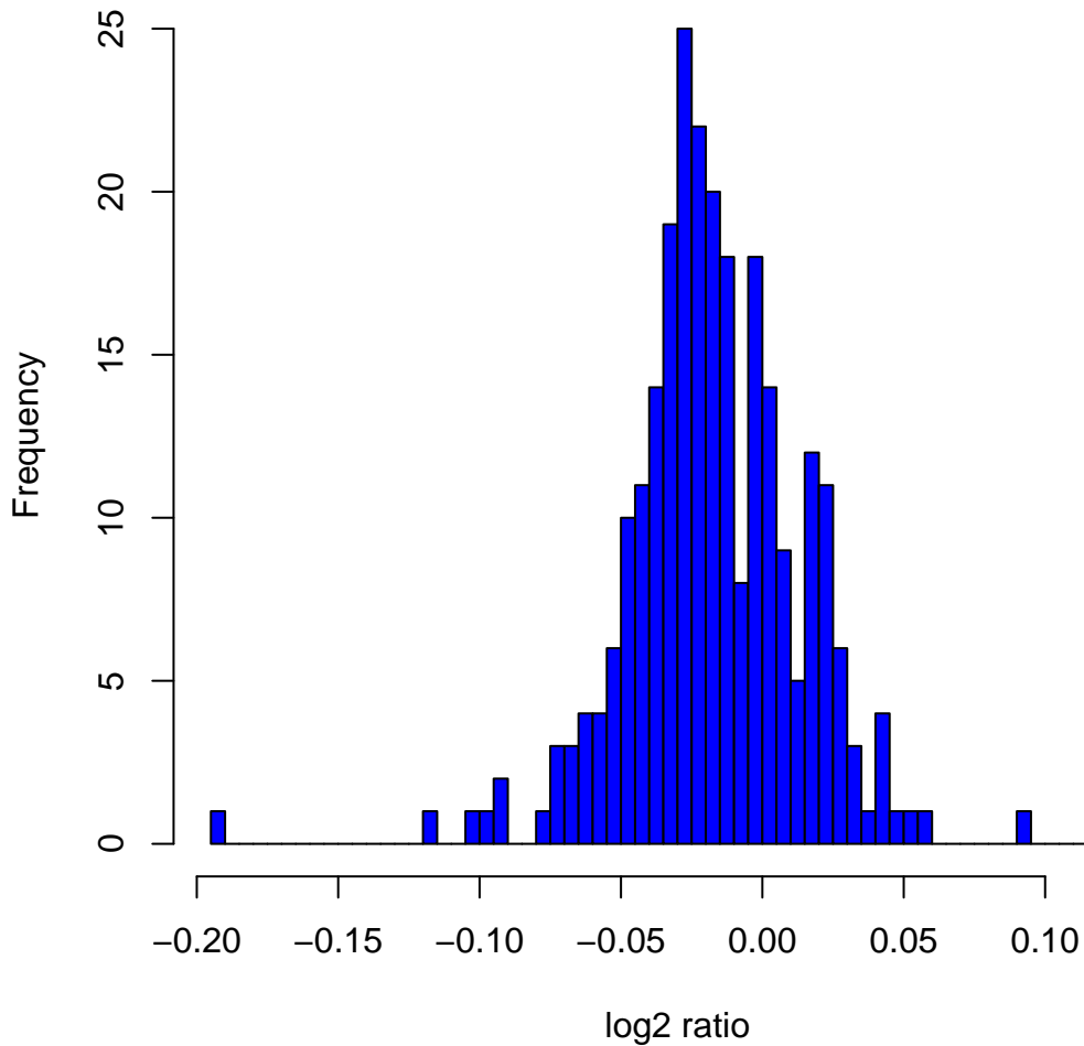
Histogram of log2ratios in 270 HapMap samples at clone Chr7tp-12C10
