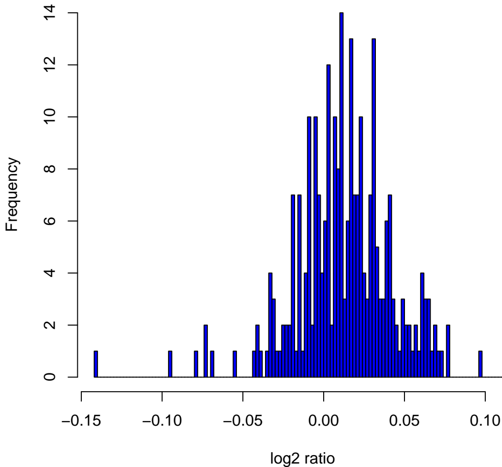
Histogram of log 2 ratios in 270 HapMap samples at clone Chr7tp-12E5
