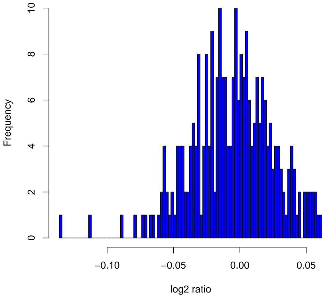
Histogram of log2ratios in 270 HapMap samples at clone Chr7tp-13A10
