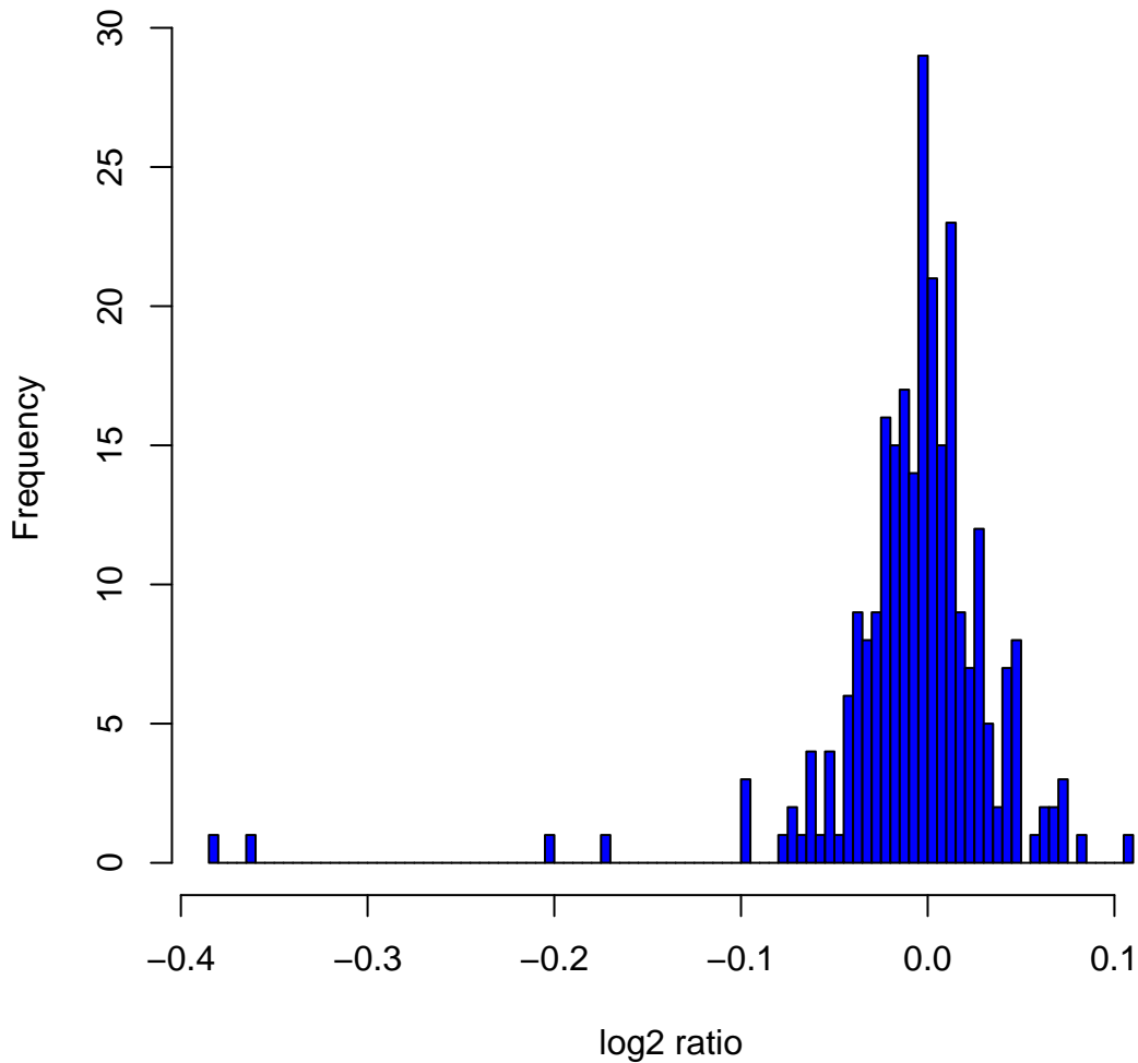
Histogram of log2ratios in 270 HapMap samples at clone Chr7tp-13C10
