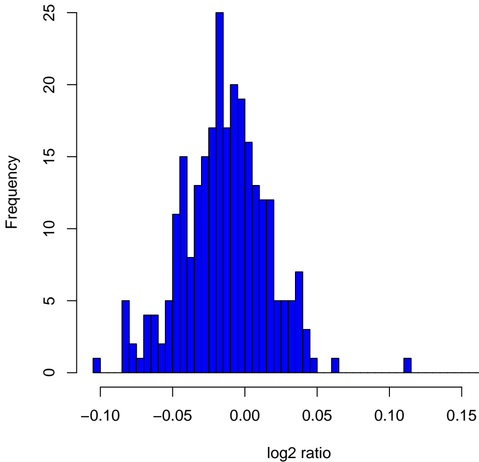
Histogram of log2ratios in 270 HapMap samples at clone Chr7tp-14D10
