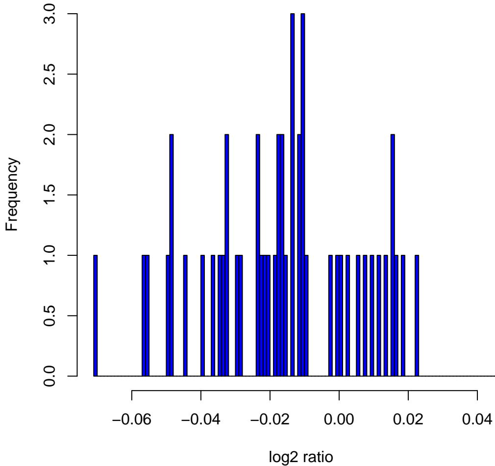
Histogram of log 2 ratios in 270 HapMap samples at clone Chr7tp-14D4
