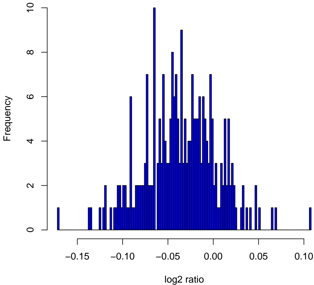
Histogram of log2ratios in 270 HapMap samples at clone Chr7tp-14E12
