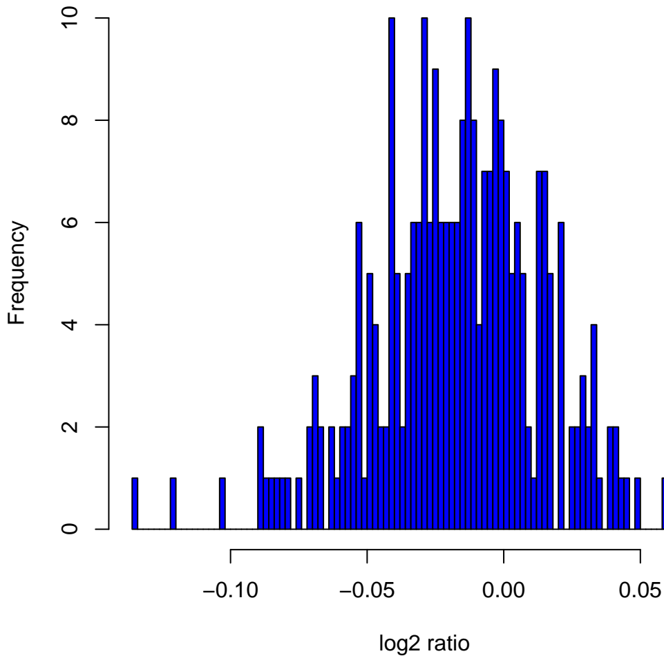
Histogram of \log_2 ratios in 270 HapMap samples at clone Chr7tp-14F2
