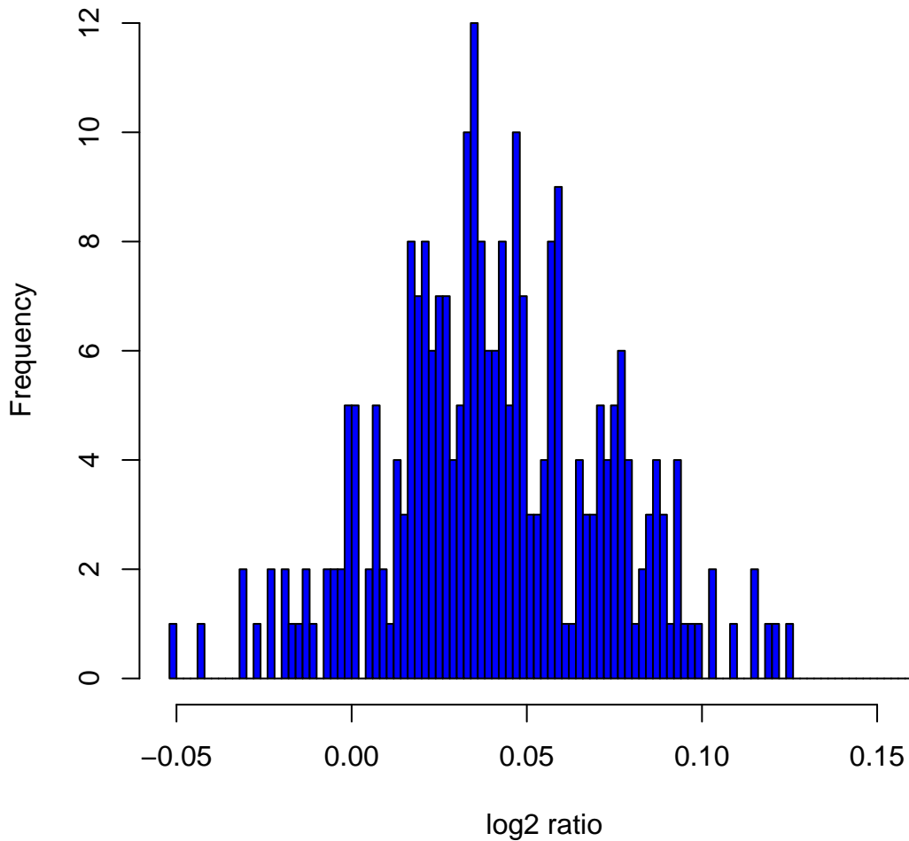
Histogram of log2ratios in 270 HapMap samples at clone Chr7tp-16A12
