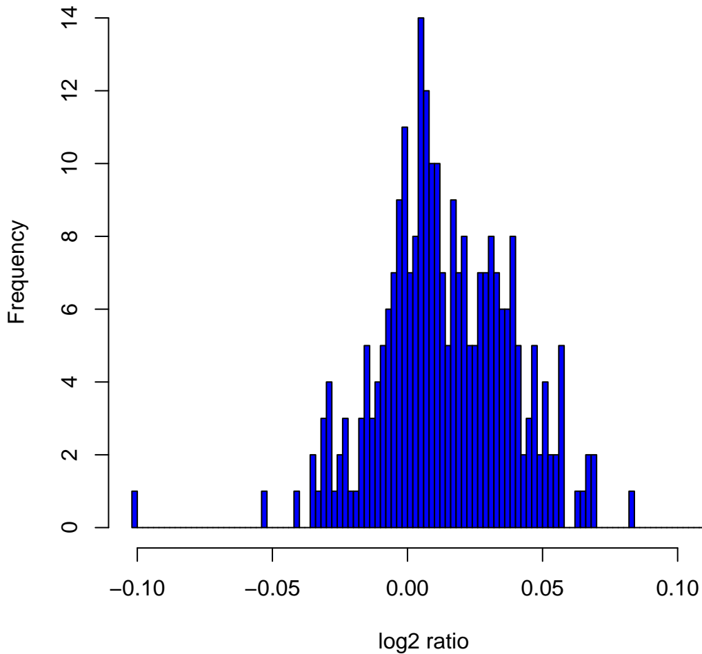
Histogram of log 2 ratios in 270 HapMap samples at clone Chr7tp-17A4
