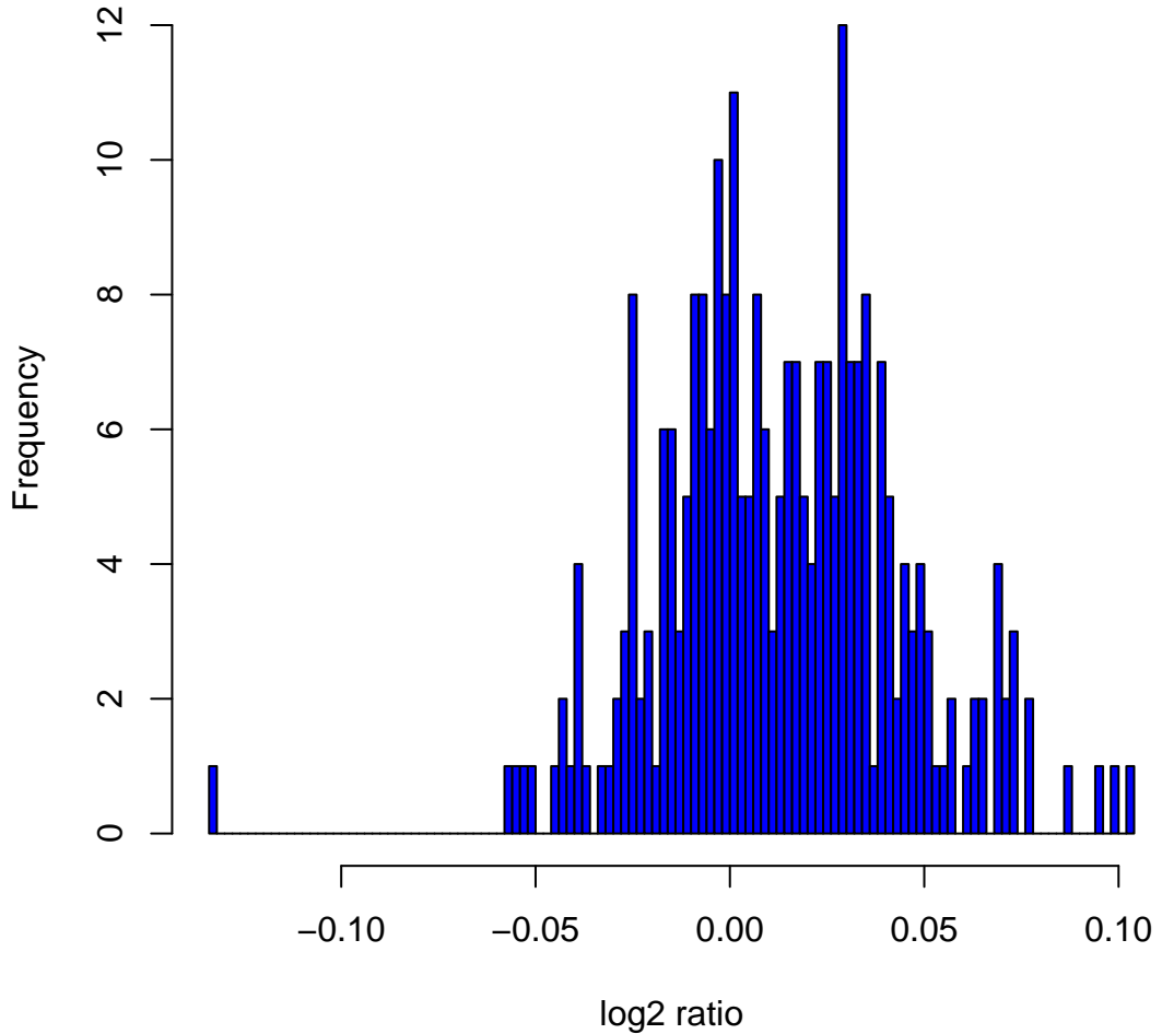
Histogram of log 2 ratios in 270 HapMap samples at clone Chr7tp-17B4
