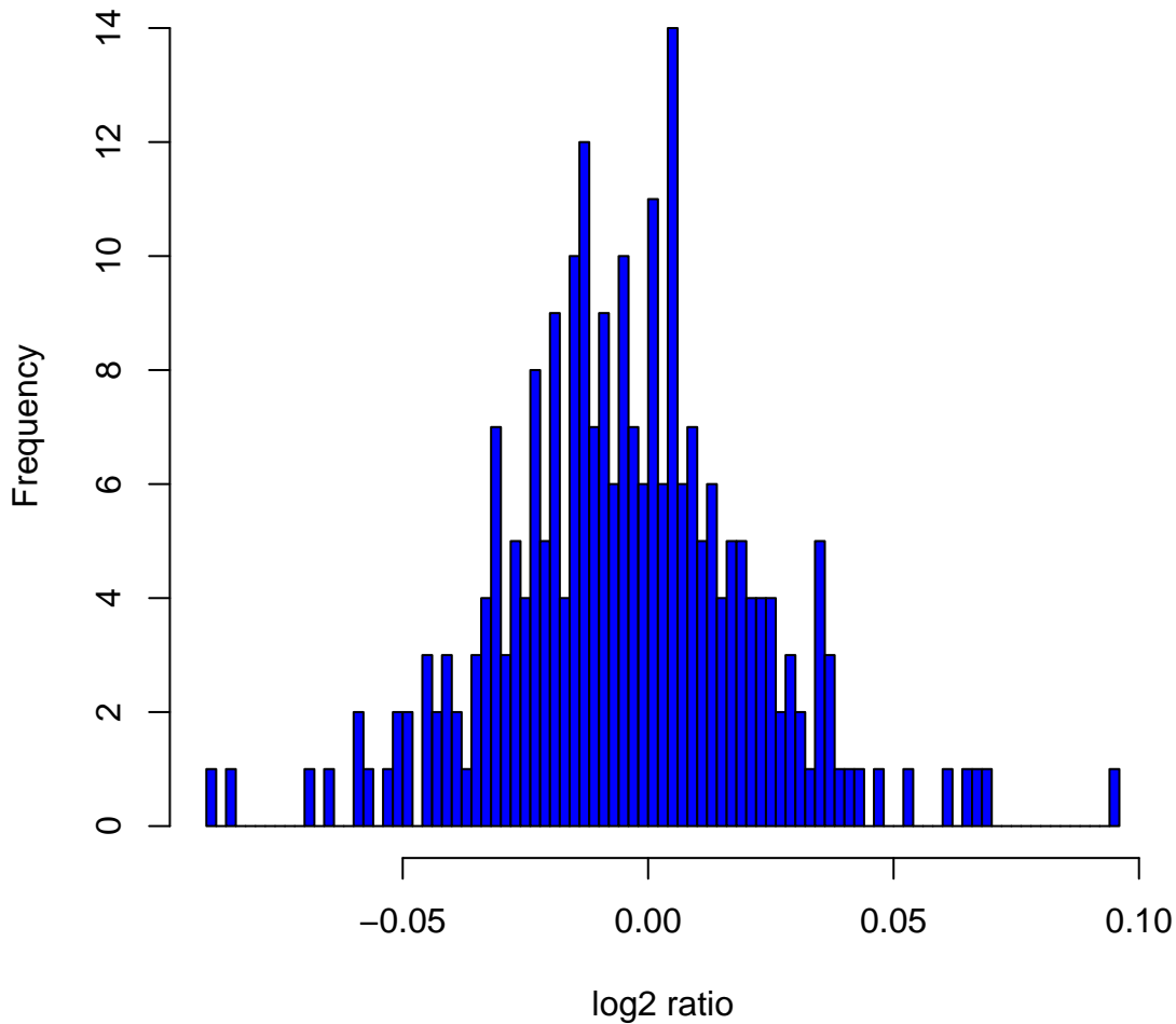
Histogram of log 2 ratios in 270 HapMap samples at clone Chr7tp-17B5
