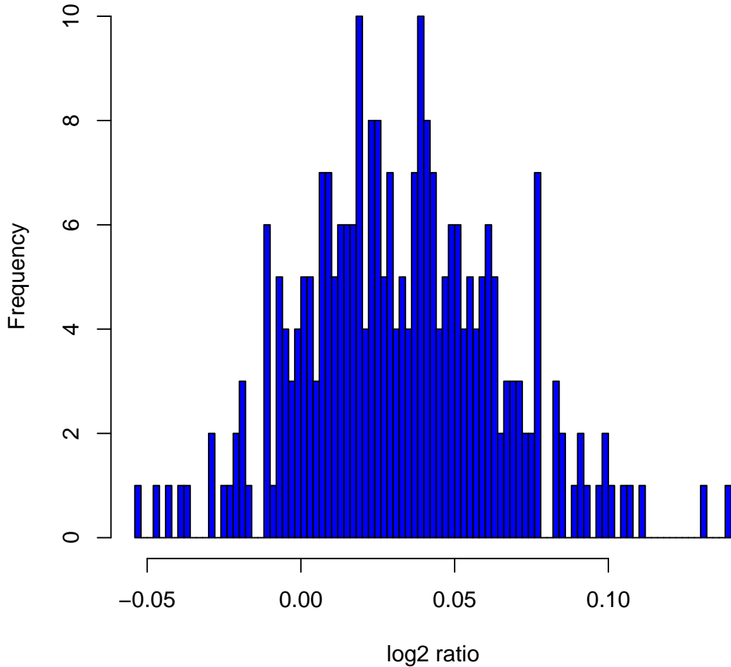
Histogram of log 2 ratios in 270 HapMap samples at clone Chr7tp-17F1
