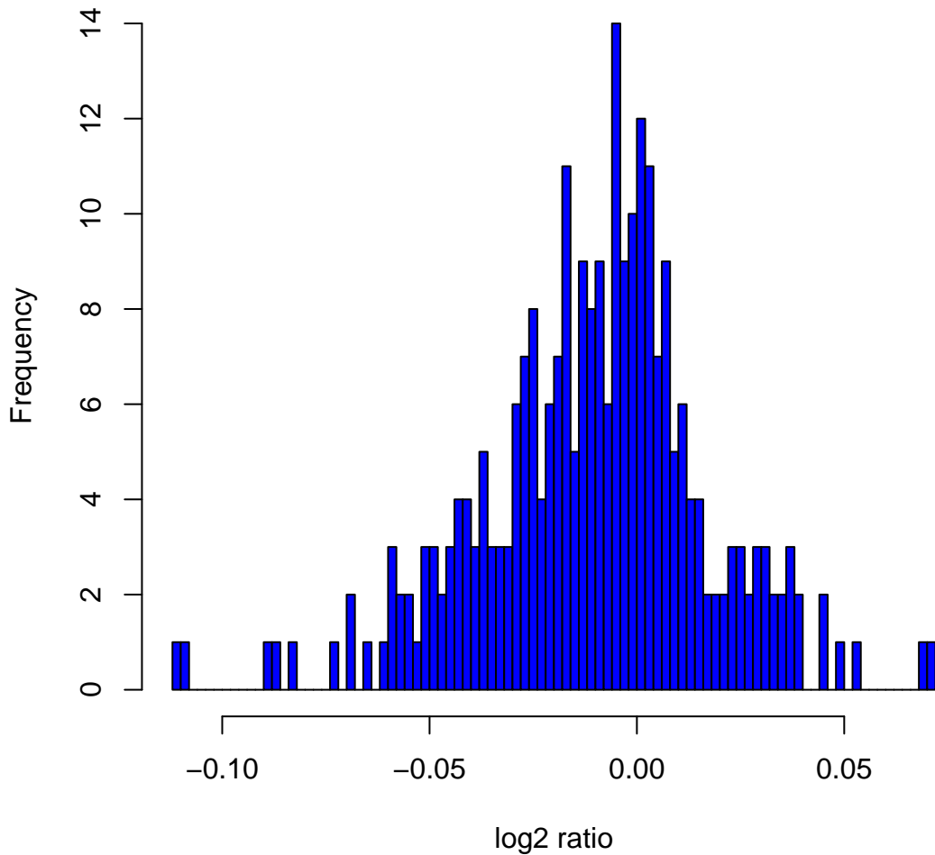
Histogram of log2ratios in 270 HapMap samples at clone Chr7tp-17H11
