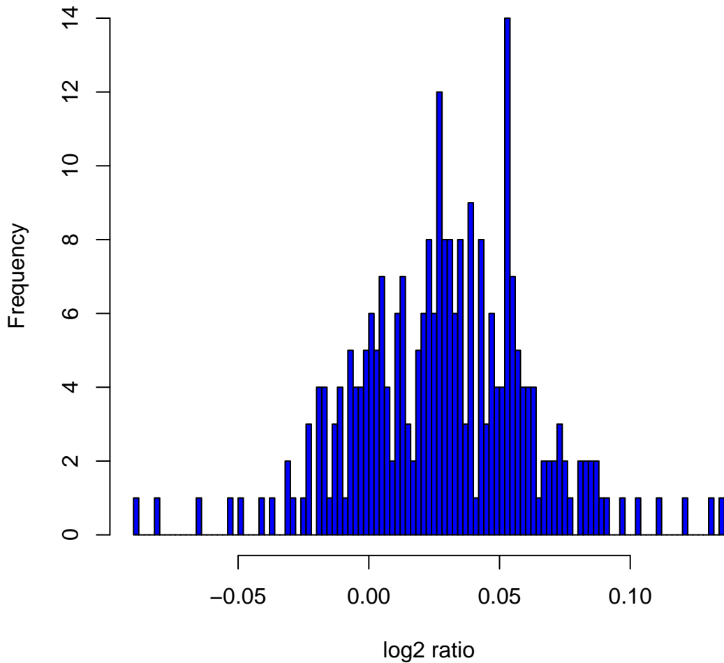
Histogram of log 2 ratios in 270 HapMap samples at clone Chr7tp-18A2
