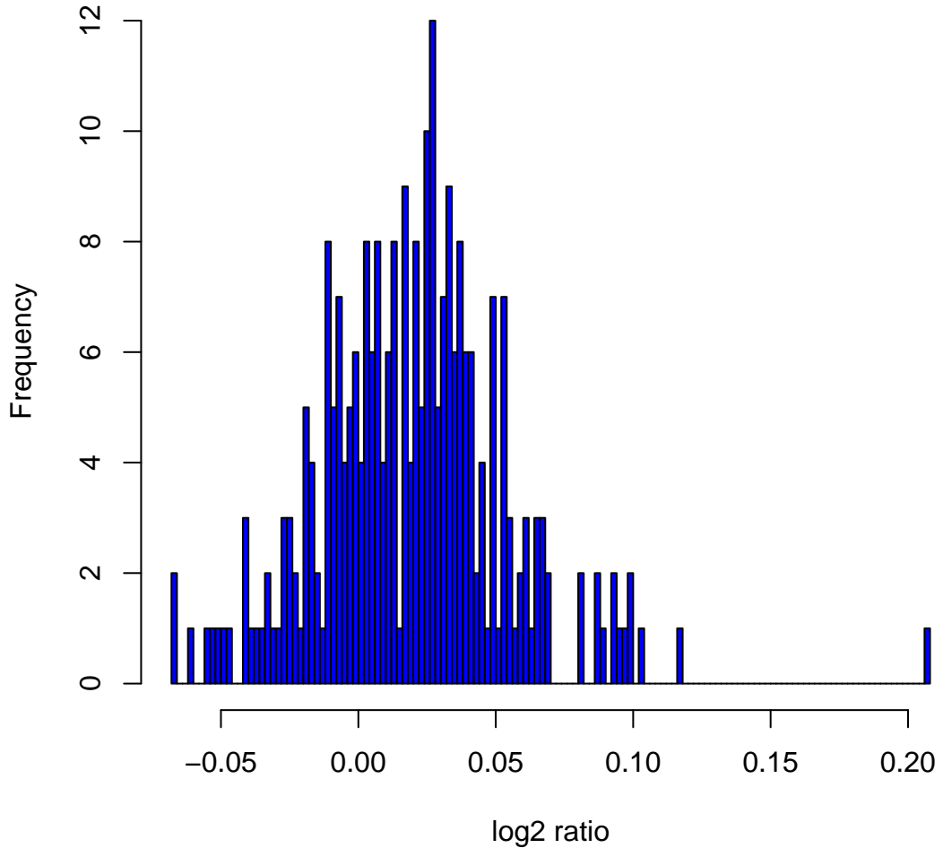
Histogram of log 2 ratios in 270 HapMap samples at clone Chr7tp-18B4
