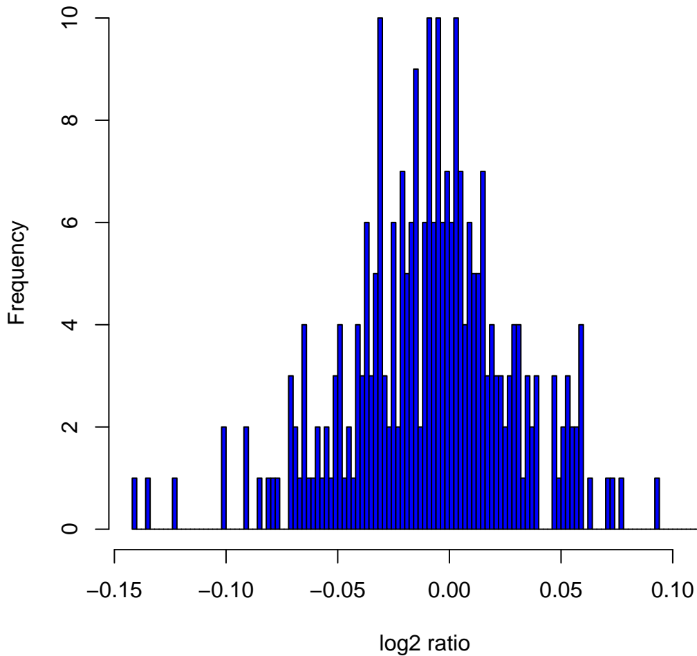
Histogram of \log_2 ratios in 270 HapMap samples at clone Chr7tp-18F4
