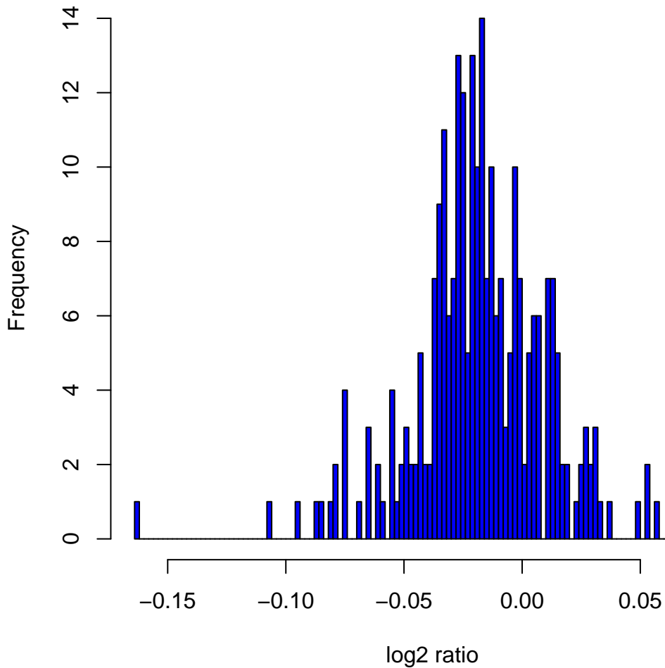
Histogram of log2ratios in 270 HapMap samples at clone Chr7tp-19B10
