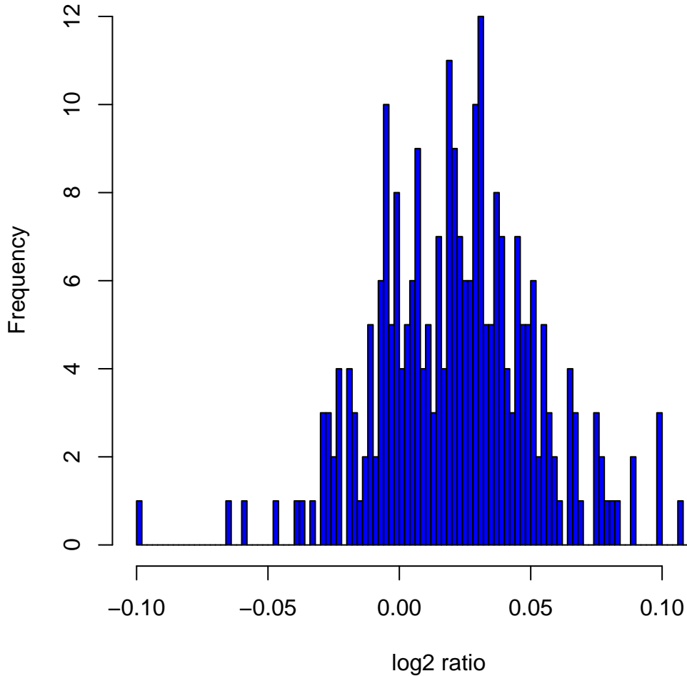
Histogram of log 2 ratios in 270 HapMap samples at clone Chr7tp-19D4
