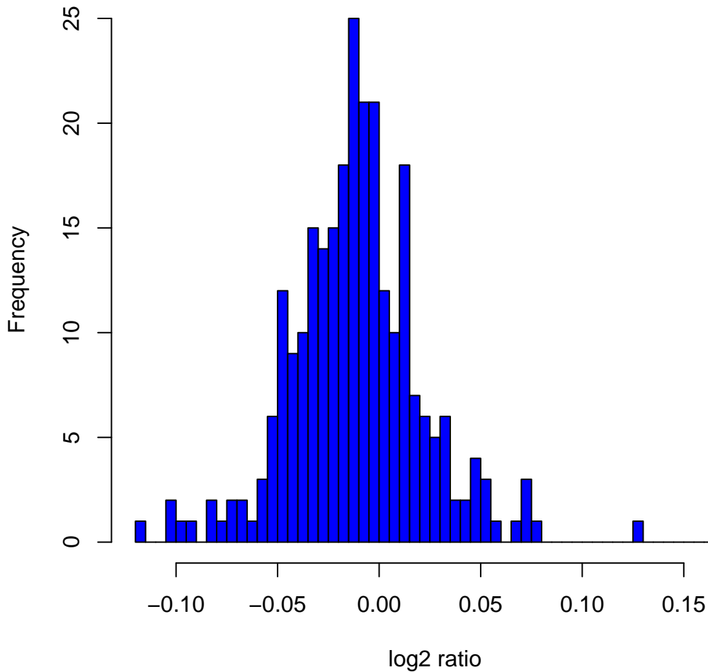
Histogram of log2ratios in 270 HapMap samples at clone Chr7tp-19F11
