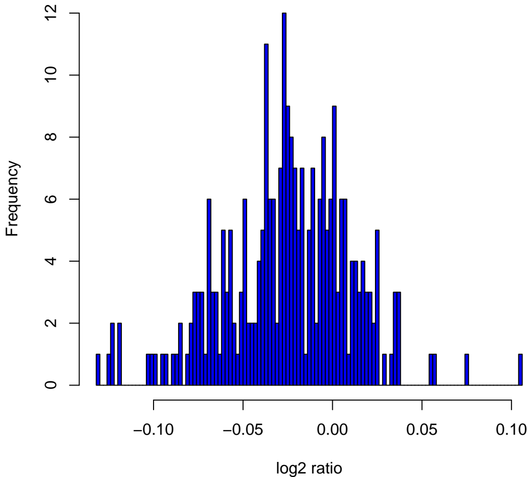
Histogram of log 2 ratios in 270 HapMap samples at clone Chr7tp-19G3
