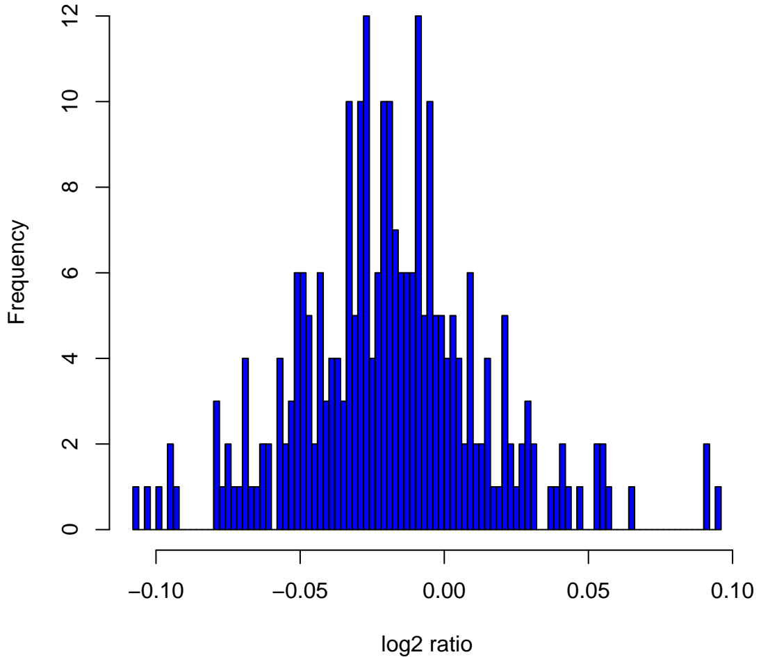
Histogram of log2ratios in 270 HapMap samples at clone Chr7tp-19H11
