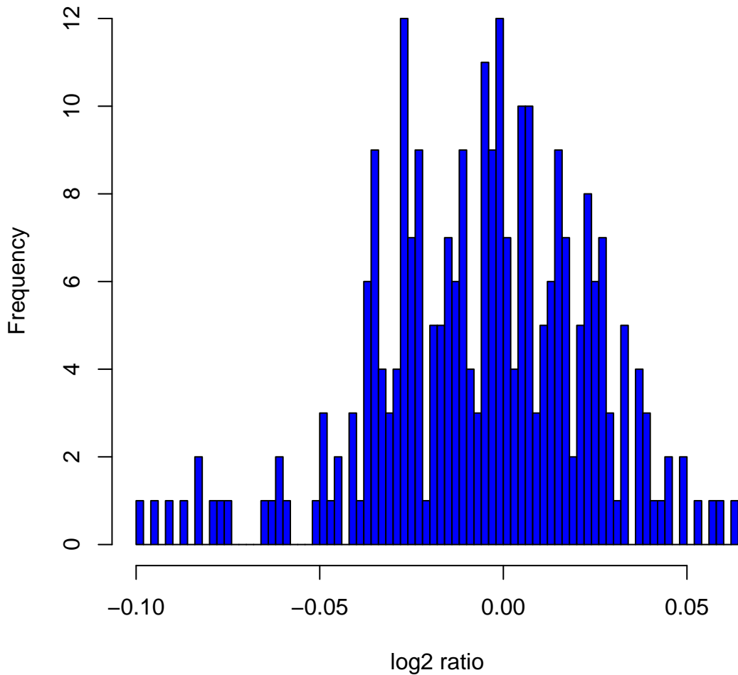
Histogram of log 2 ratios in 270 HapMap samples at clone Chr7tp-1A12
