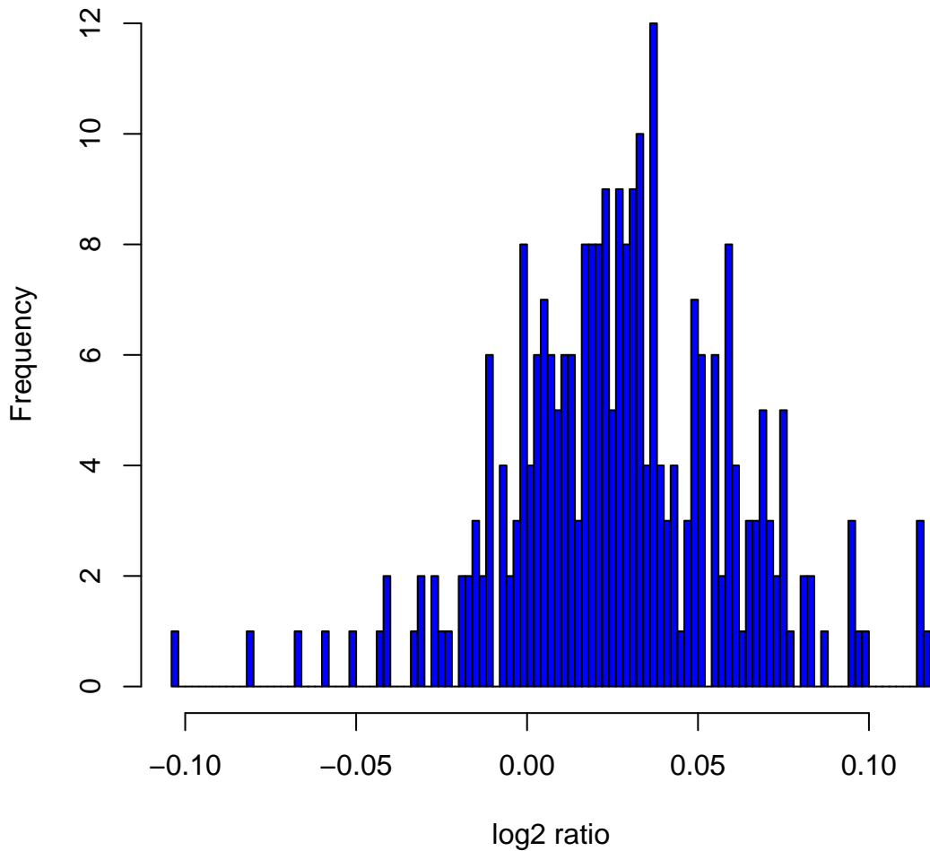
Histogram of log 2 ratios in 270 HapMap samples at clone Chr7tp-1A4
