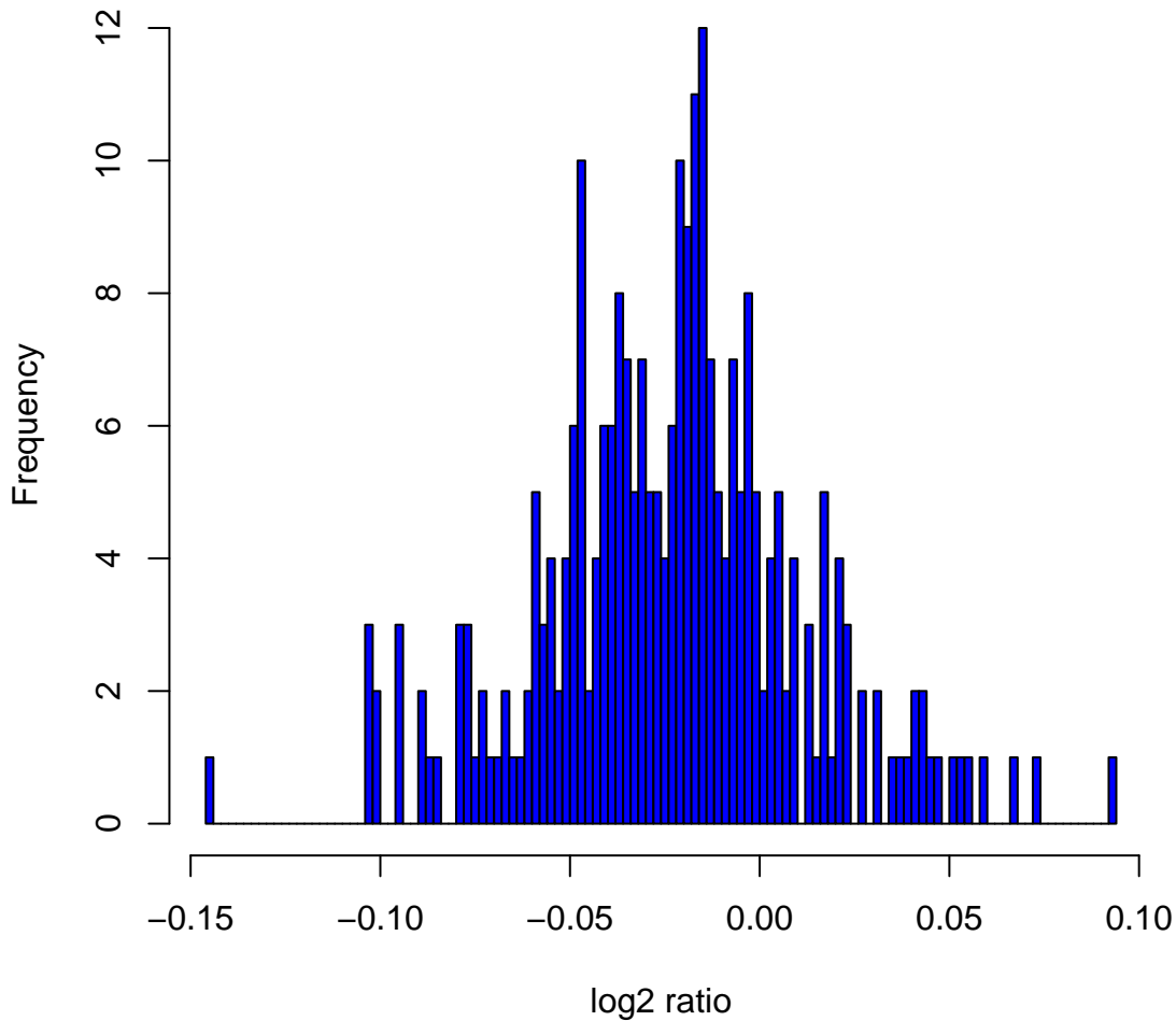
Histogram of log 2 ratios in 270 HapMap samples at clone Chr7tp-1A8
