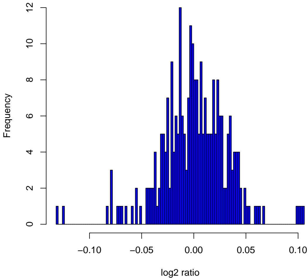
Histogram of \log_2 ratios in 270 HapMap samples at clone Chr7tp-1B5
