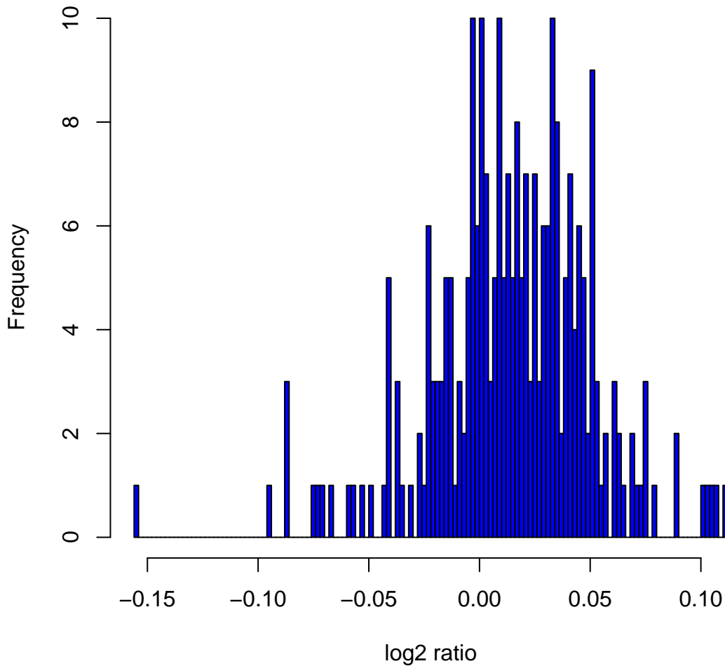
Histogram of log 2 ratios in 270 HapMap samples at clone Chr7tp-1B8
