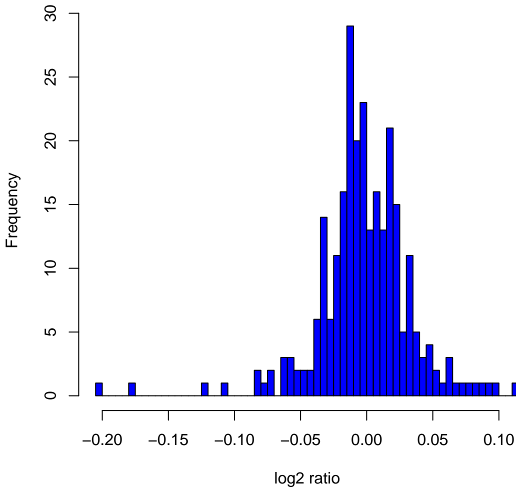
Histogram of log 2 ratios in 270 HapMap samples at clone Chr7tp-1C12
