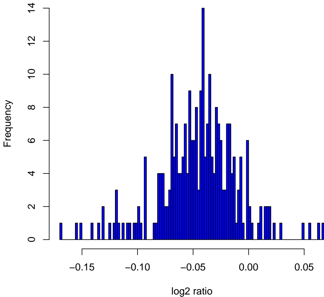
Histogram of log 2 ratios in 270 HapMap samples at clone Chr7tp-1E10
