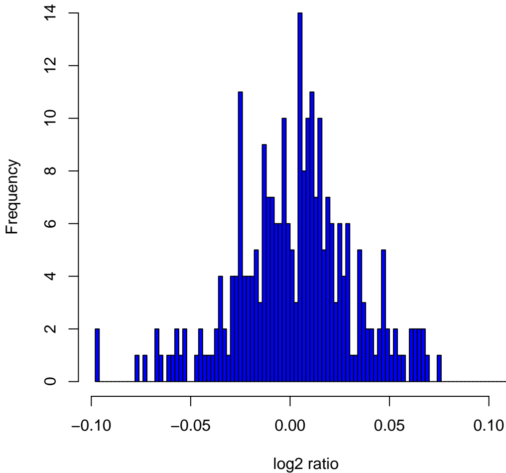
Histogram of log2ratios in 270 HapMap samples at clone Chr7tp-1F5
