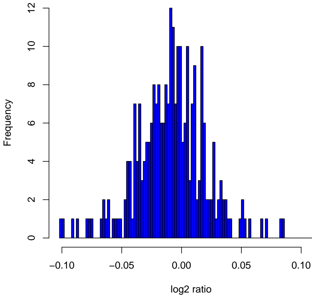
Histogram of log2ratios in 270 HapMap samples at clone Chr7tp-1H4
