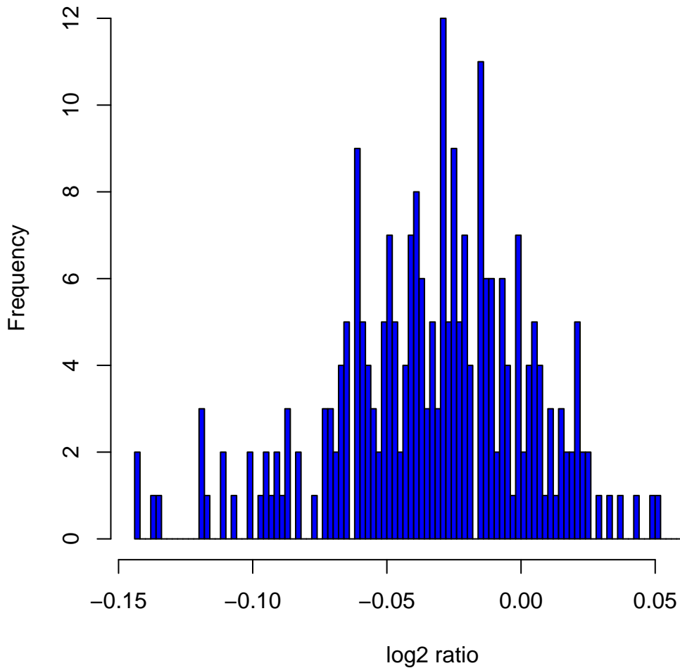
Histogram of \log_2 ratios in 270 HapMap samples at clone Chr7tp-1H7
