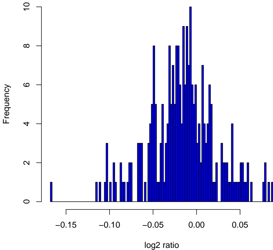
Histogram of log2ratios in 270 HapMap samples at clone Chr7tp-20B10
