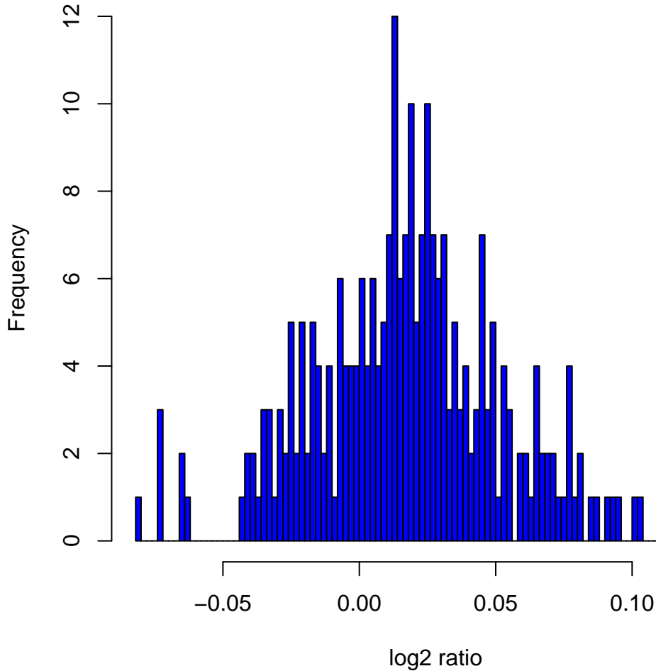
Histogram of log2ratios in 270 HapMap samples at clone Chr7tp-20B11
