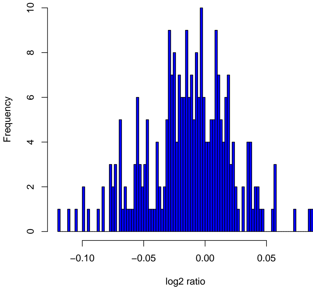
Histogram of log2ratios in 270 HapMap samples at clone Chr7tp-20B12
