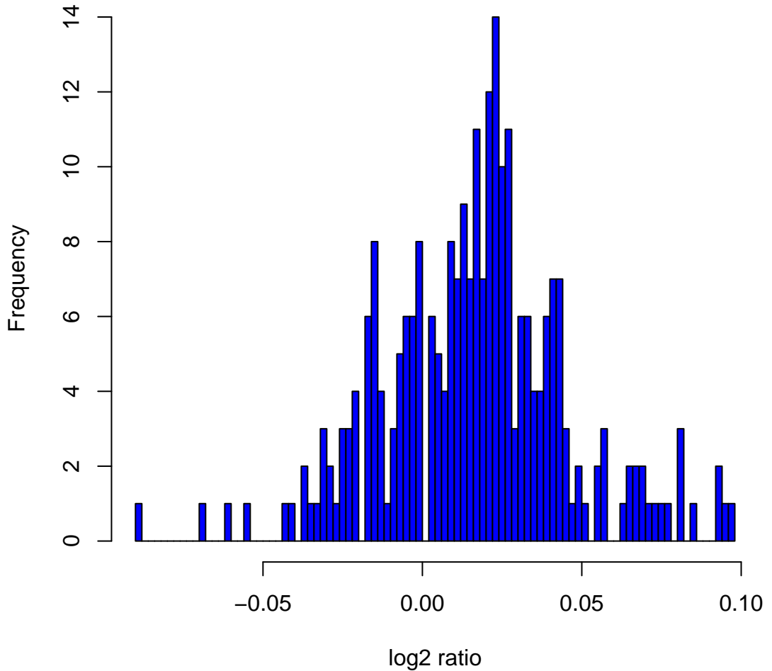
Histogram of log 2 ratios in 270 HapMap samples at clone Chr7tp-20B5
