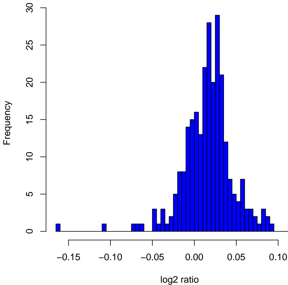
Histogram of log 2 ratios in 270 HapMap samples at clone Chr7tp-20D6
