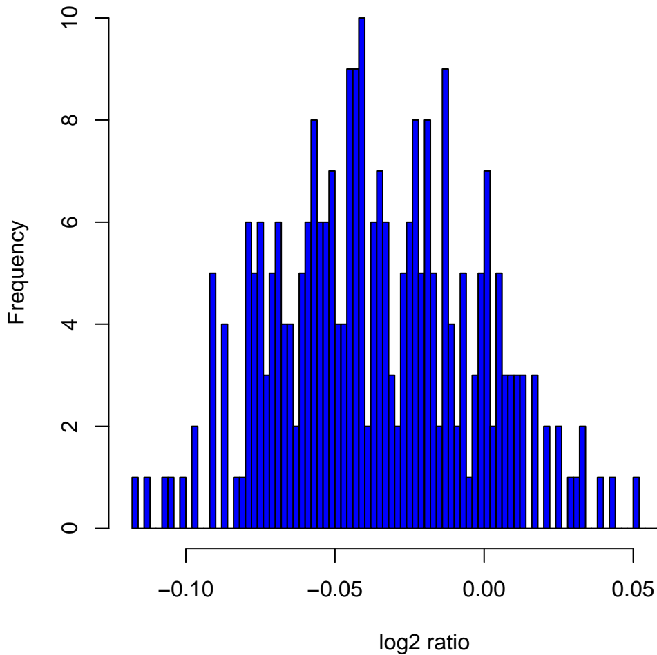
Histogram of \log_2 ratios in 270 HapMap samples at clone Chr7tp-20E8
